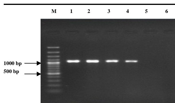
Figure 1. PCR amplification of the lipL41 gene for detection of pathogenic serovars of leptospires. M: 100 bp DNA ladder; lane1: positive control, L. Sejroe hardjo; lane 2: Positive control, L. Pomona ; lane3: L. Canicola (RTCC2805); lane4: L. Canicola (RTCC2824); lane5: L. biflexa ; lane 6: negative control
