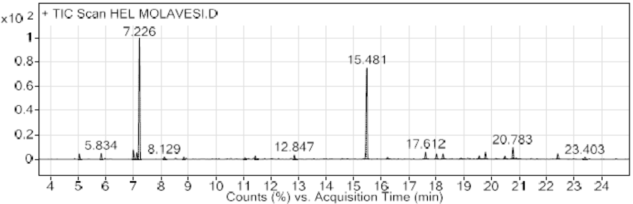
Figure 2) Chromatogram of cardamom essential oil by GC-MS method.
