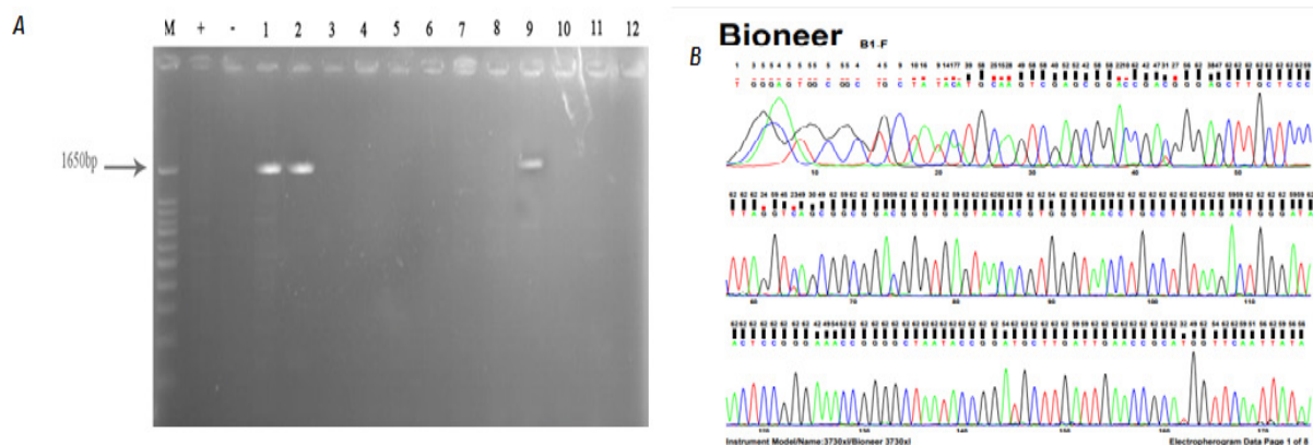
Figure 2) PCR results of celA genes: 2A: C+: positive control, C -: negative control (distilled water), and Wells 1 to 12: Streptomyces strains, 2b: the result of sequencing and BLAST of the amplified gene
